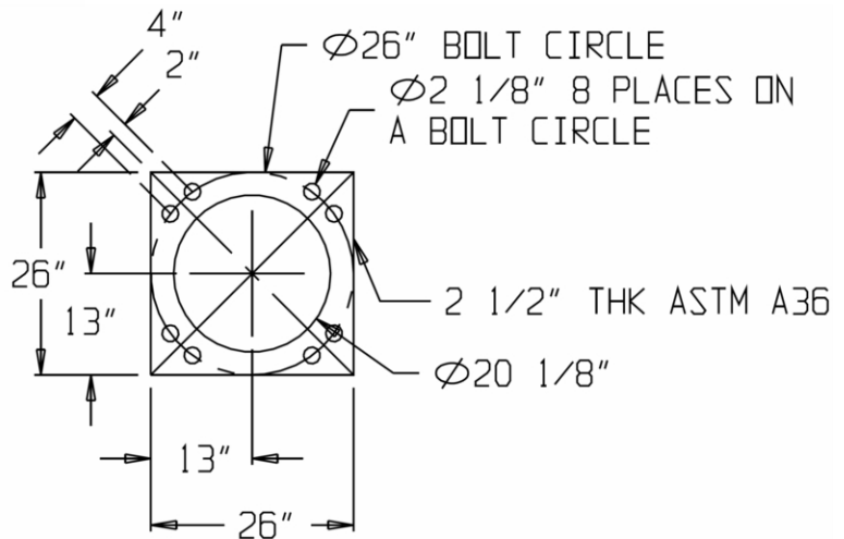
BASE PLATE DETAIL
